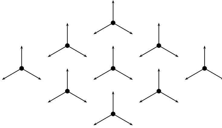
Figure 1 : Optimal azimuth in a regular hexagonal grid
