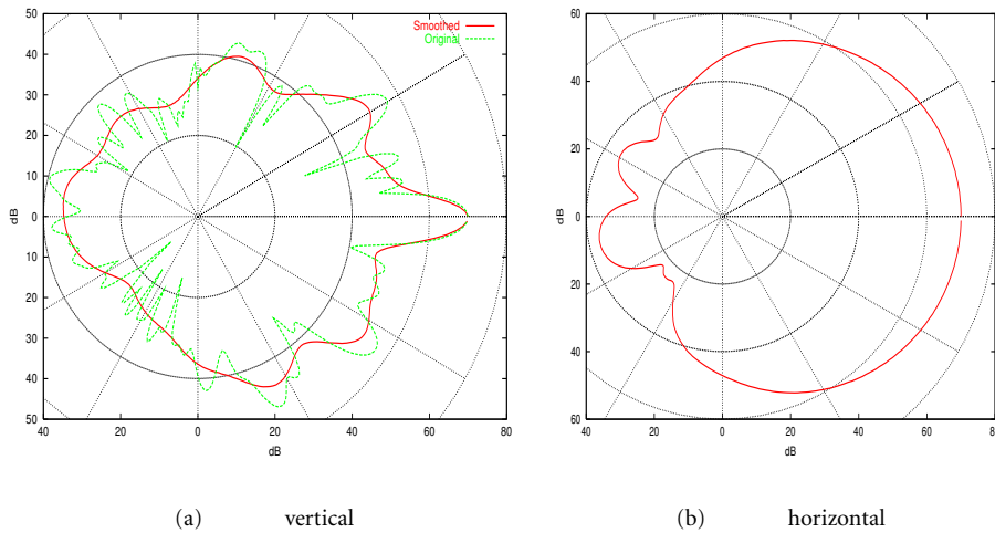
Figure 1 : Antenna diagrams
