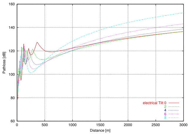
Figure . : Pathloss change depending on tilt
