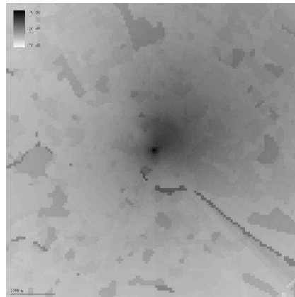
(b) Berlin, M predictor with 100 m resolution height and clutter data
