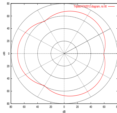
Figure 5.10: Tripled horizontal antenna diagram
