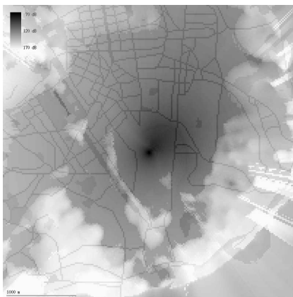
(c) Lisbon, M predictor with 100 m resolution height, clutter and merged vectorized street data
